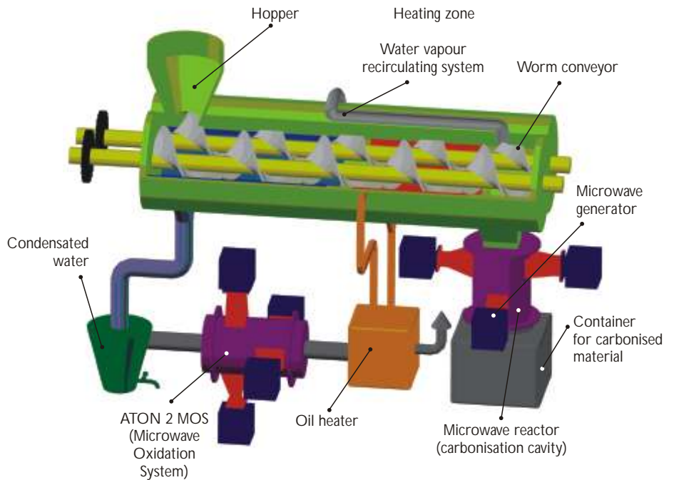
Figure 2: Diagram of a system for organic waste carbonization.
